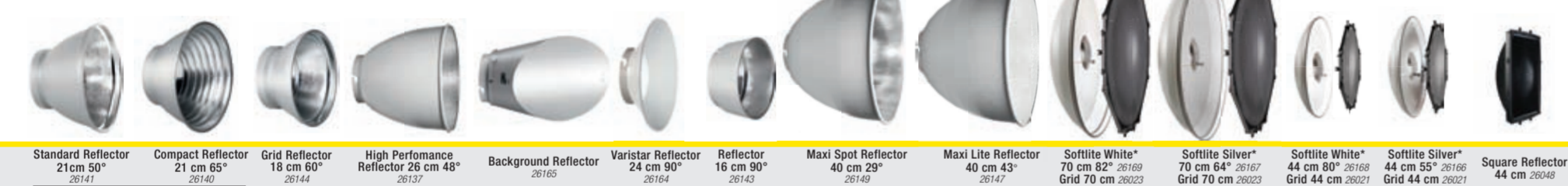
Standard Reflector 21 cm 50° 26141 Compact Reflector 21 cm 65° 26140 Grid Reflector 18 cm 60° 26144 High Performance Reflector 26 cm 48° 26137 Background Reflector 26165 Varistar Reflector 24 cm 90° 26164 Reflector 16 cm 90° 26143 Maxi Spot Reflector 40 cm 29° 26149 Maxi Lite Reflector 40 cm 43° 26147 Softlite White* 70 cm 82° 26169 Grid 70 cm 26023 Softlite Silver* 70 cm 64° 26167 Grid 70 cm 26023 Softlite White* 44 cm 80° 26168 Grid 44 cm 26021 Softlite Silver* 44 cm 55° 26166 Grid 44 cm 26021 Square Reflector 44 cm 26048 *Each Softlite reflector includes a deflector set
